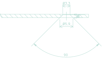
Countersink hole detail
